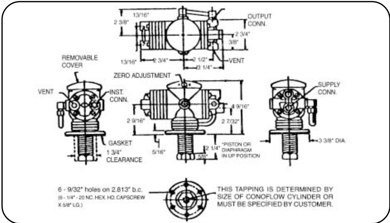
For Certified Dimensional Data, refer to Drawings A50-50 (GC32)
