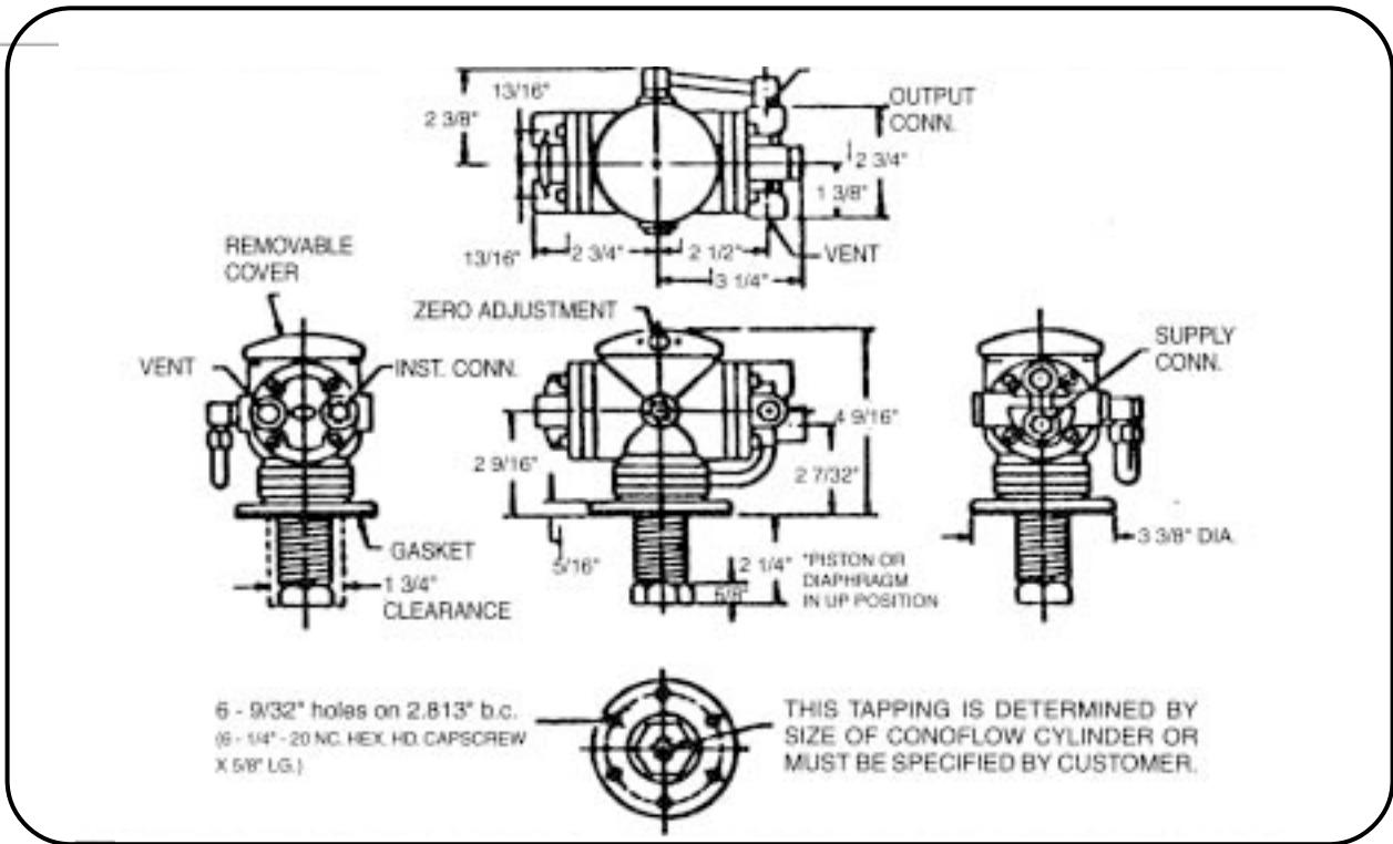
For Certified Dimensional Data, refer to Drawings A50-49 (GC31)
